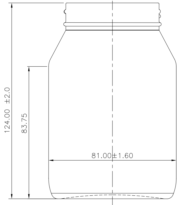
PARTING VIEW
